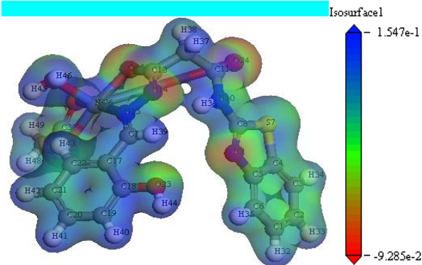
[Ni(HBT)(H 2 O)(OAc)].3H 2 O
