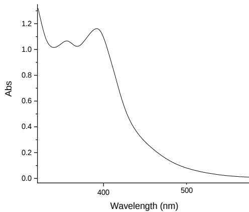
Figure 3S. UV of (A) [\text{Cu}(\text{BT})(\text{H}_2\text{O})_2].2\text{H}_2\text{O} , (B) [\text{Co}(\text{HBT})(\text{H}_2\text{O})(\text{OAc})].2\text{H}_2\text{O} , and (C) [\text{Ni}(\text{HBT})(\text{H}_2\text{O})(\text{OAc})].3\text{H}_2\text{O}
