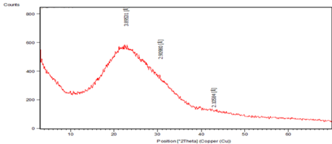
Figure 7S. XRD of (A)[Cu(L)(H 2 O) 2 ].2H 2 O complex
