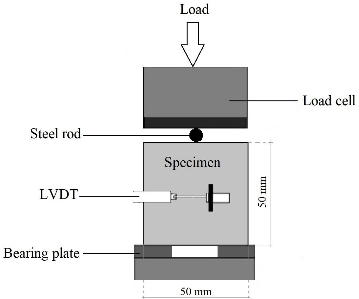
Fig. S4. Setup for creating microcrack on cubic specimens.
