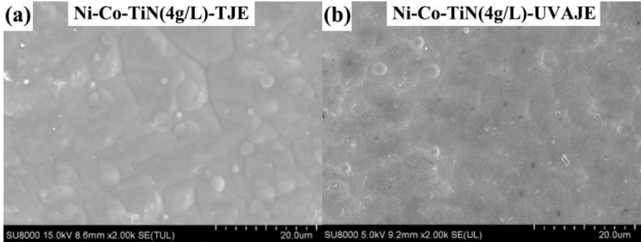
Fig. S8 SEM images of the different Ni-Co-TiN coatings after salt spray test.
