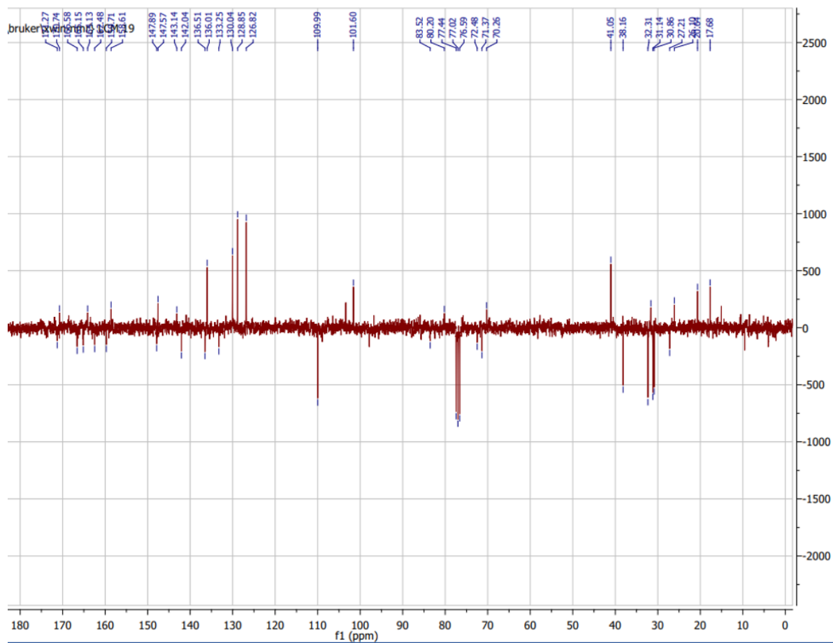
Fig.3S. ^{13}\text{C} Decoupled ^1\text{H} NMR spectrum
