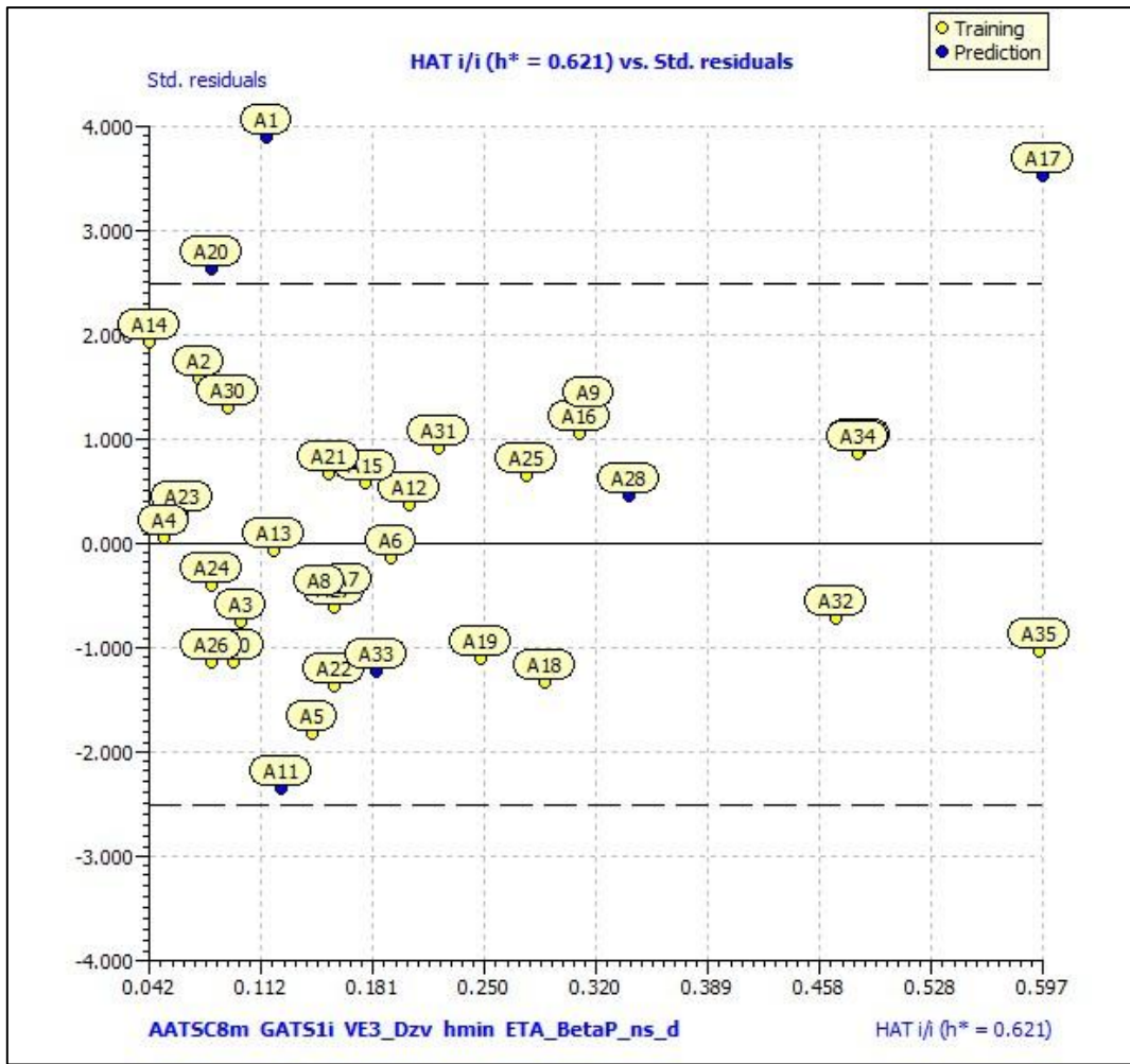
Fig.S1. Applicability domain plot for the Model 1
