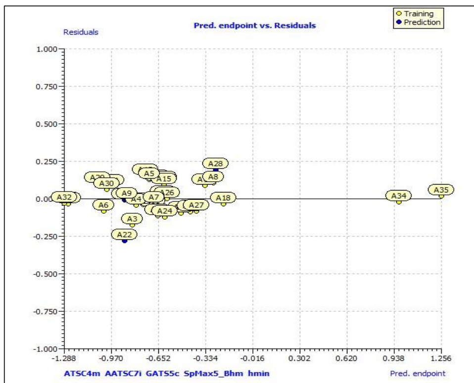
Fig.S2. Plot between the predicted activity and the residual values of the Model 2
