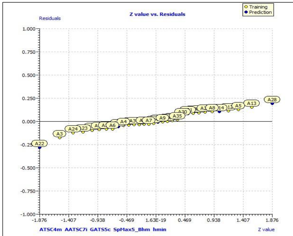
Fig.S3. Plot between the Z values against the residuals of the Model 2
