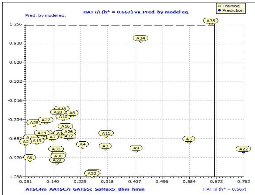
Fig.S6. Applicability Domain – Insurbia plot of the Model 2
