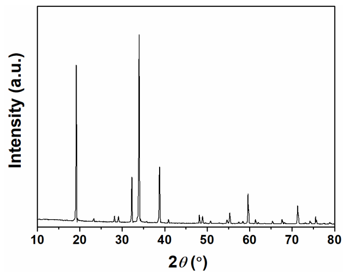
Fig. S1. XRD pattern of the dried and neutralized reaction system.
