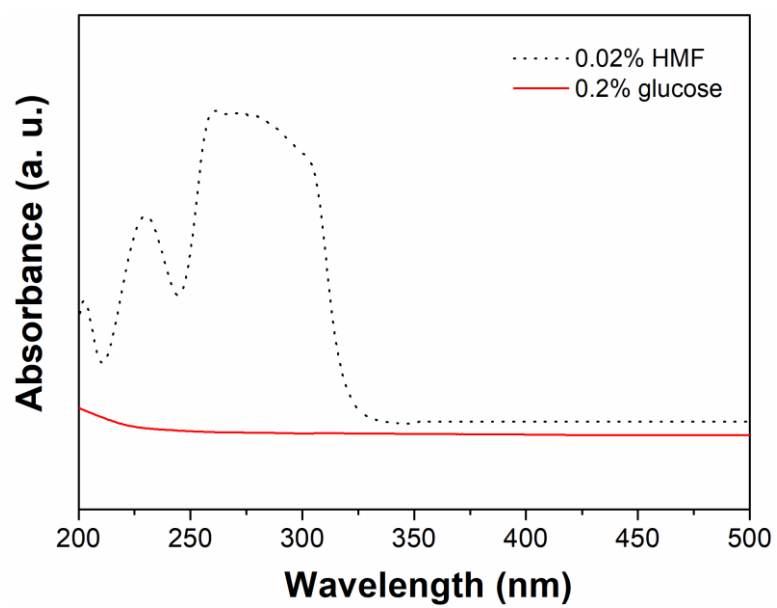
Fig. S3. UV-Vis spectra of HMF (aq) and glucose (aq).
